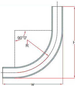
5) Duct 90° Street Lighting Long Radius Bend 4"
