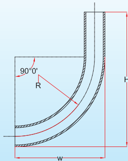
6) Duct 90° Street Lighting Long Radius Bend 3"
