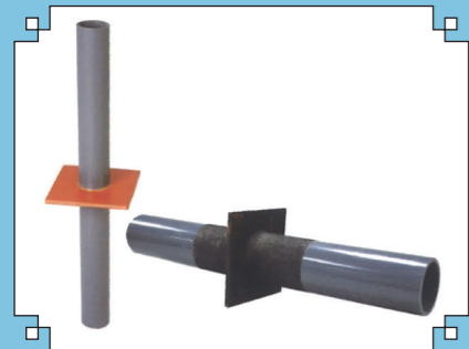
Puddle Flange Soil/Drainage/Pressure
